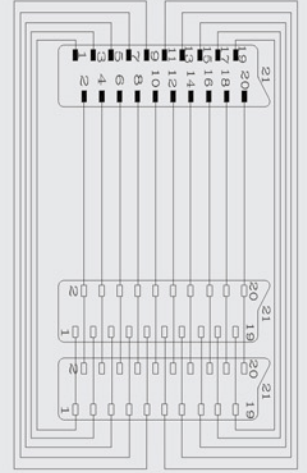
21P Scart Plug - 2 x 21P Scart Jacks slimmer box design, 2-Way Scart splitter
