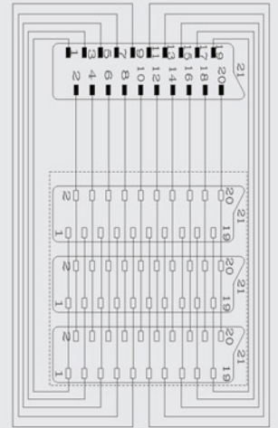
21P Scart Plug - 3 x 21P Scart Jacks slimmer box design, 3-Way Scart splitter
