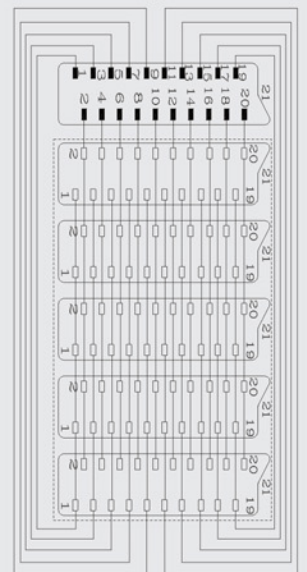
21P Scart Plug - 5 x 21P Scart Jacks slimmer box design, 5-Way Scart splitter
